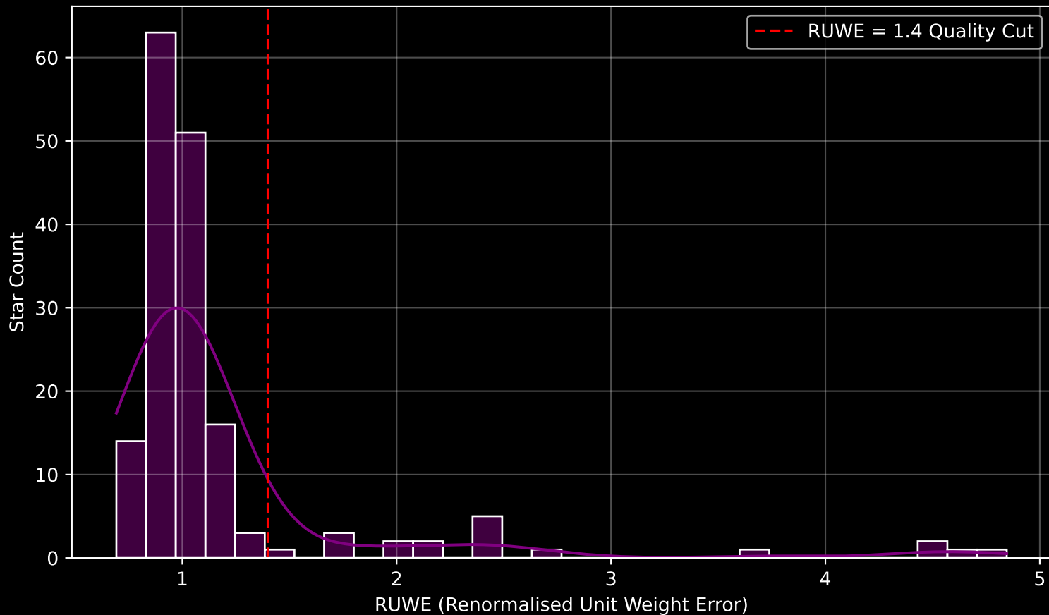
GAPOGEE DR17 Field [CVZ_OB07_btx] RUWE Distribution (n= 166)
