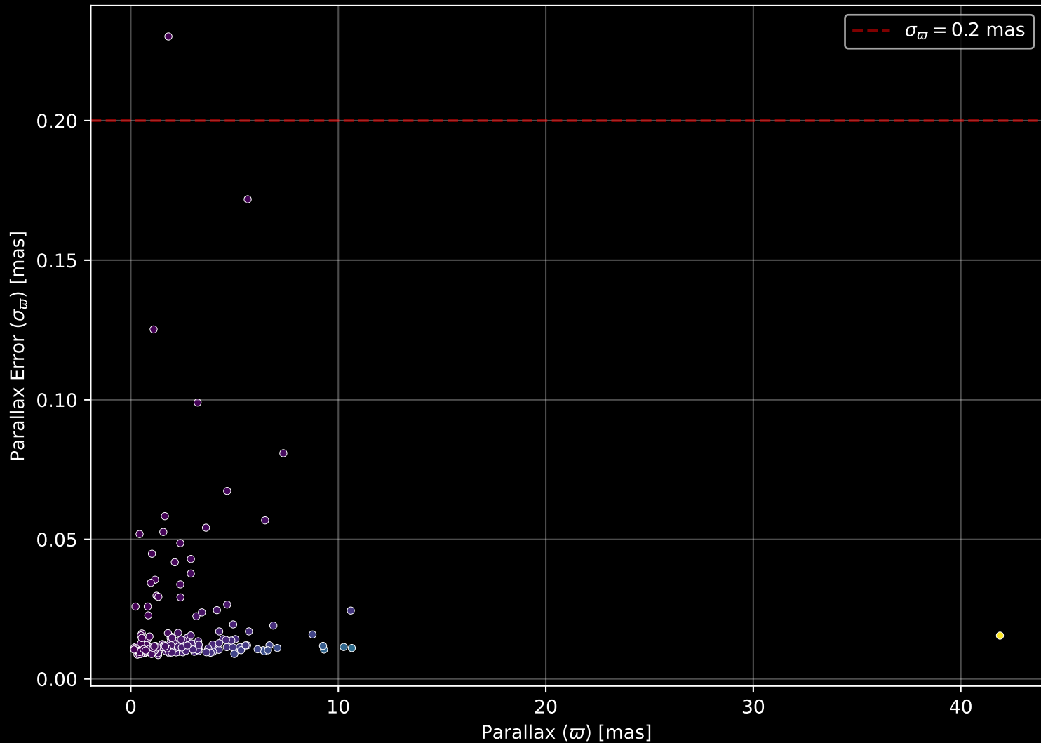
APOGEE DR17 Field: [CVZ_OB07_btx] Parallax Quality (n= 173)
