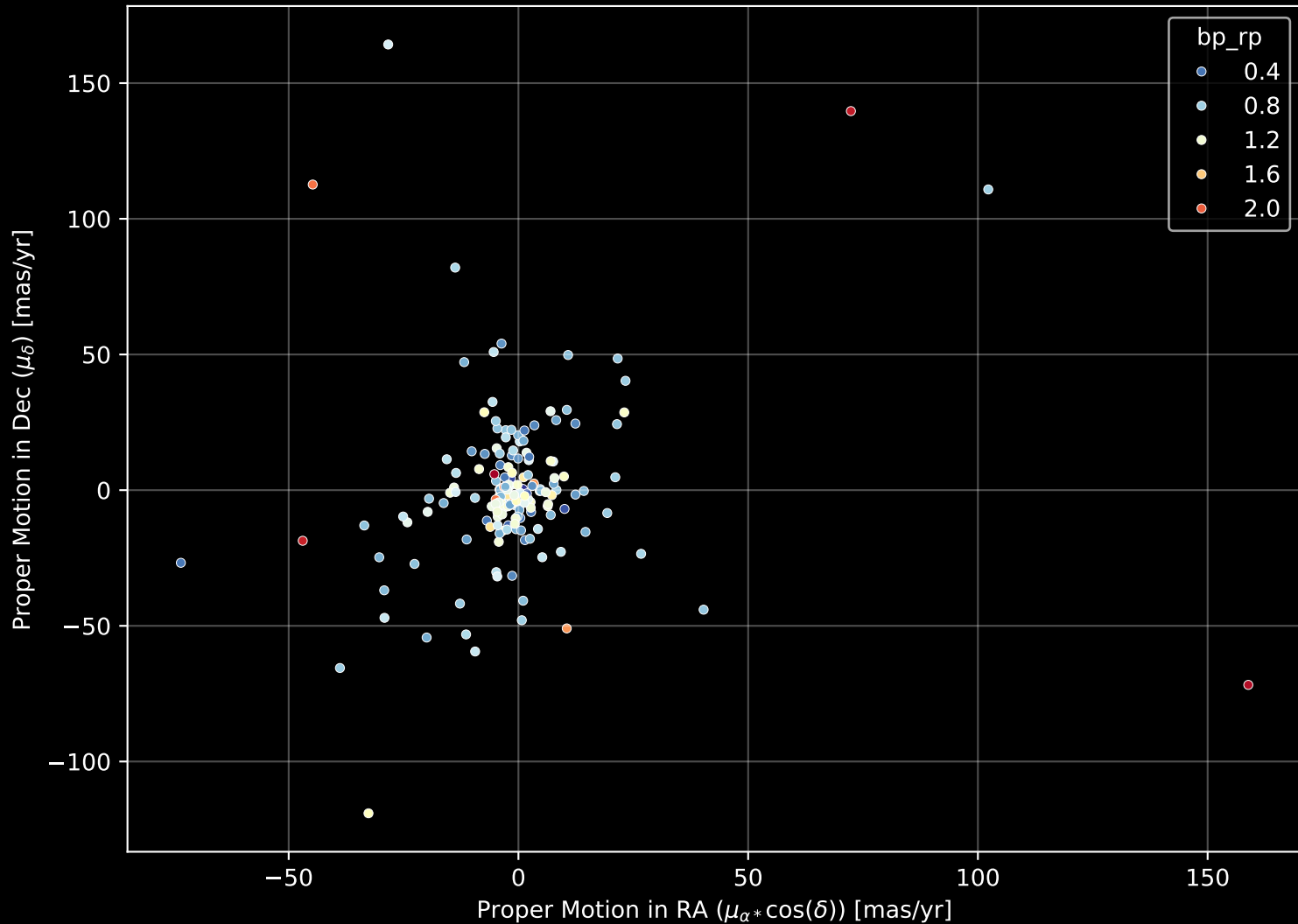
APOGEE DR17 Field: [CVZ_OB07_btx] Proper Motion Diagram (n= 173)
