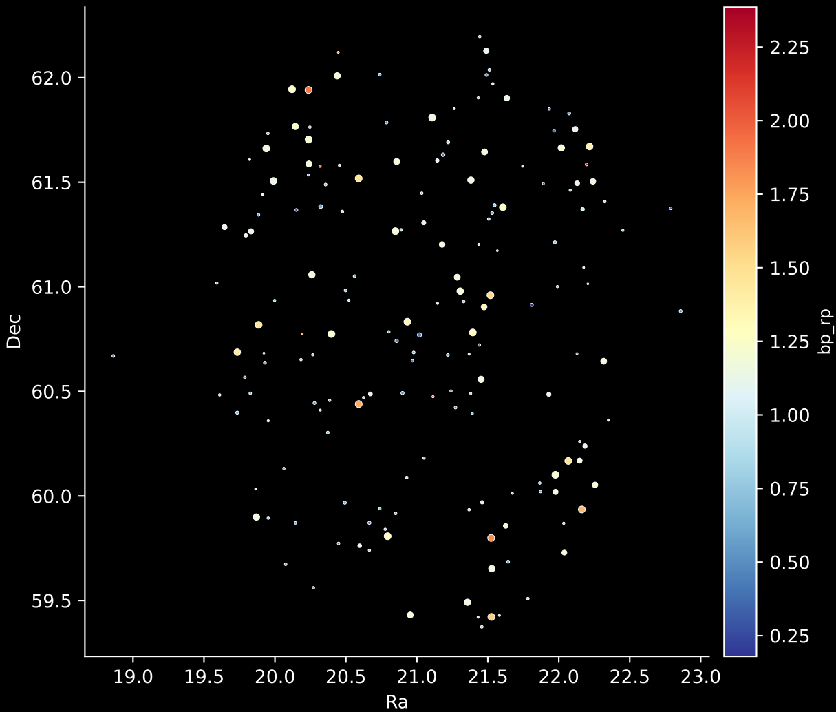
APOGEE DR17 Field: [CVZ_OB07_btx] Stars: 173
