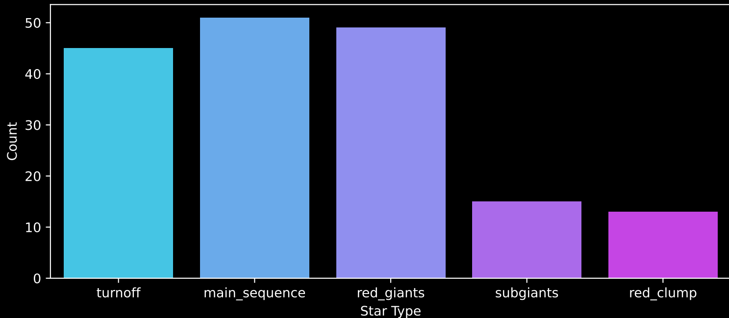
APOGEE DR17 Field: [CVZ_OB07_btx] Count plot of Star Type
