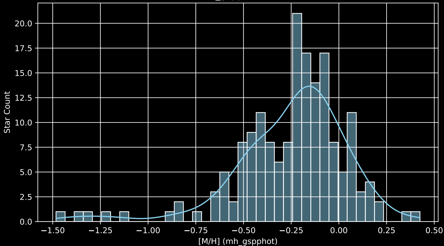
APOGEE DR17 Field: [CVZ_OB07_btx [M/H] (mh_gspphot) (n= 173)
